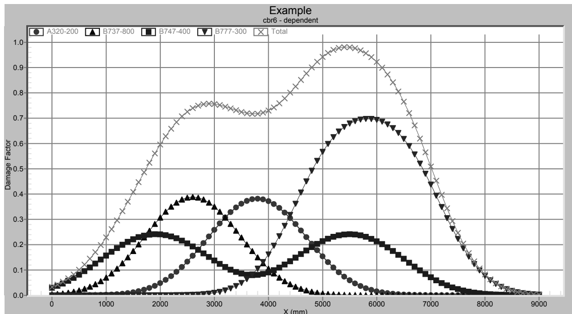
Figure 1: Sample APSDS 5.0 CDF Graph showing CDF variation across a pavement
