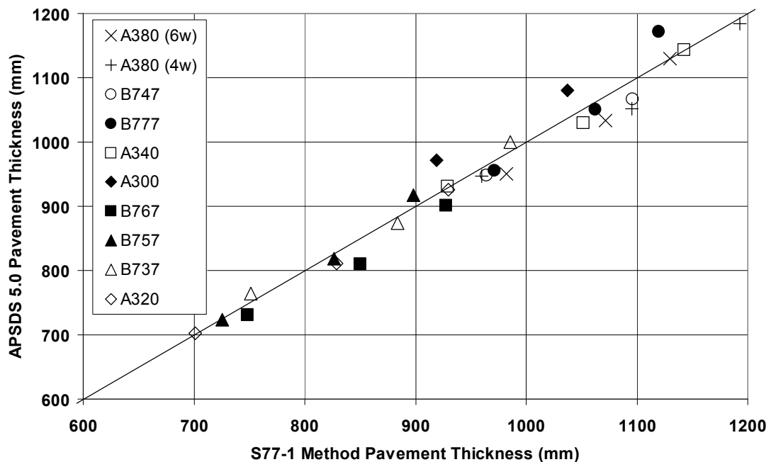
Figure 2: APSDS 5.0 pavement thickness vs. S77-1 method pavement thickness (subgrade CBR of 6%)
