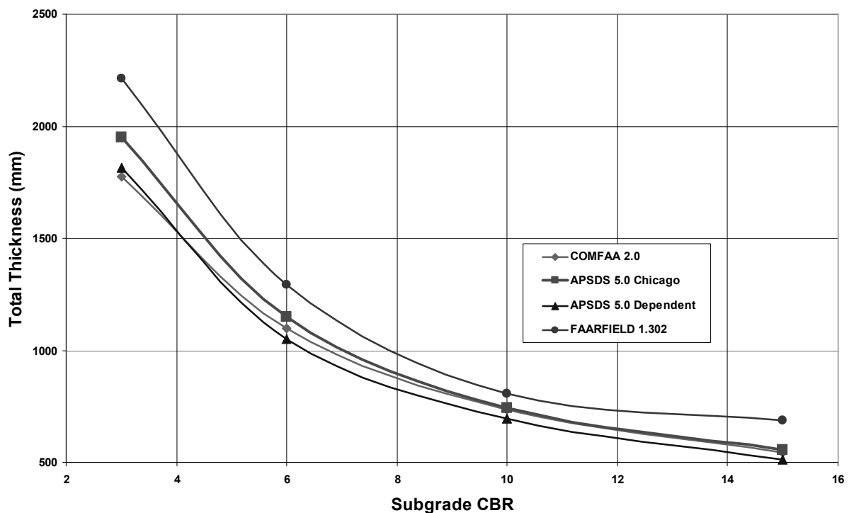
Figure 3: APSDS, COMFAA and FAARFIELD B747-400 pavement thicknesses (100,000 aircraft passes)
