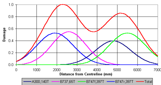
Damage graph shows damage variation across pavement.
