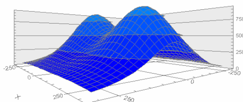
Sample Three-dimensional plot: strain pulse under dual wheels
